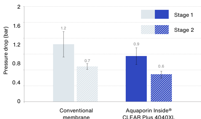
Figure 2: Pressure drop across element array
