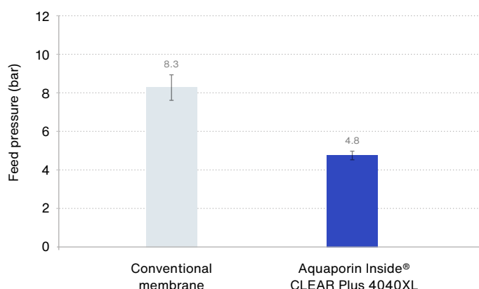
Figure 1: Feed inlet pressures
