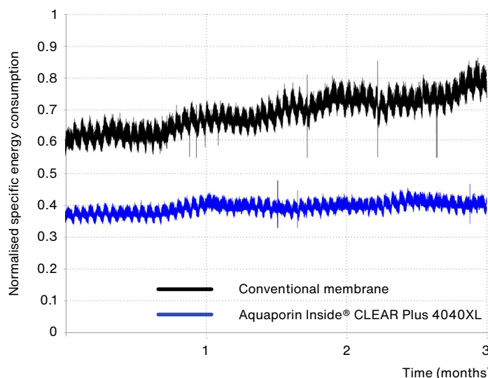
Figure 3: Trending of specific energy consumption
